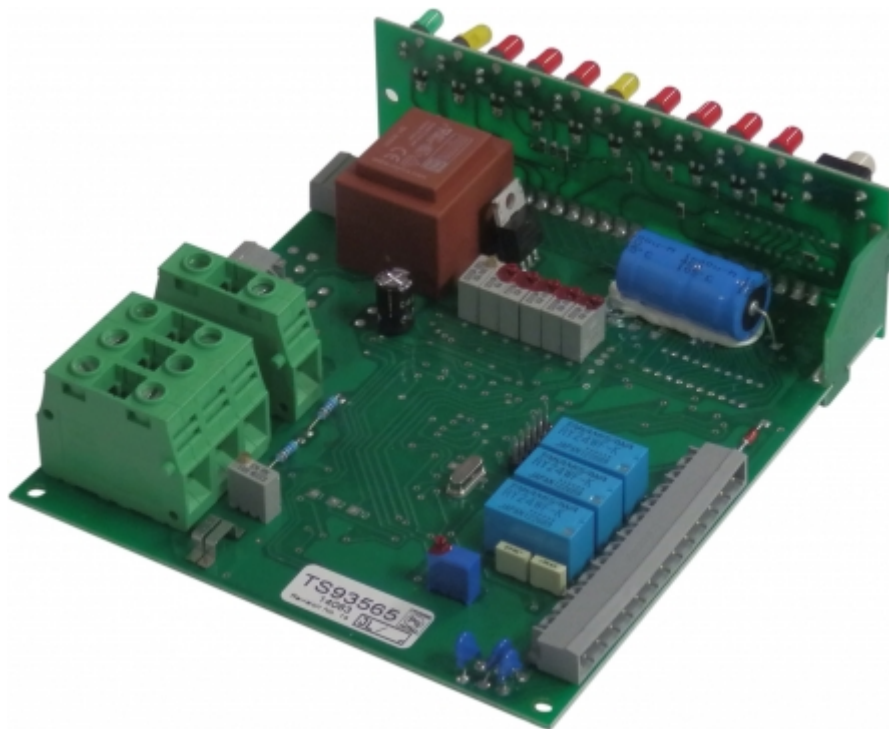
Central Unit Board for TKT6x Central Battery Systems (TS93565)
